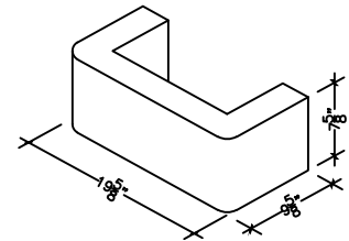
10" X 8" X 20" COLUMN COVER
