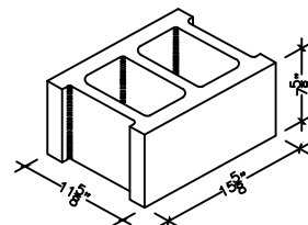
12" X 8" X 16" HOLLOW STRETCHER (ALSO IN 18")
