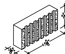
4" X 8" X 16" SOLID STRETCHER SPLIT RIB
