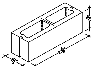
8" X 8" X 24" HOLLOW DOUBLE CORNER SASH ( 2 HOLE )
