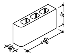
4" X 8" X 16" HOLLOW SINGLE BULLNOSE CORNER (ALSO IN 18")
