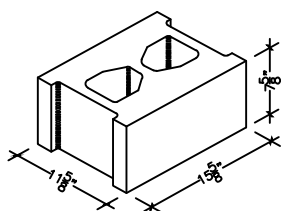
12" X 8" X 16" 75% SOLID (ALSO IN 18")
