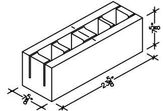
8" X 8" X 24" OPEN BOTTOM BOND BEAM ( 4 HOLE )
