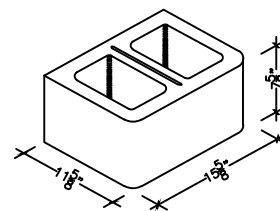
12" X 8" X 16" HOLLOW DOUBLE BULLNOSE (ALSO IN 18")
