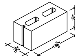
8" X 8" X 16" 75% SOLID CORNER SASH (ALSO IN 18")
