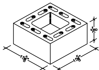
16" X 8" X 16" CHIMNEY BLOCK
