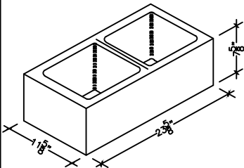
12" X 8" X 24" HOLLOW STRETCHER
