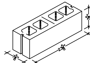
8" X 8" X 24" HOLLOW DOUBLE CORNER SASH ( 4 HOLE )
