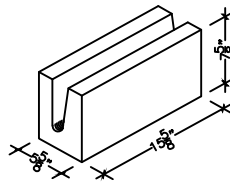
6" X 8" X 16" BOND BEAM LINTEL (ALSO IN 18")
