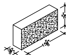
4" X 8" X 16" SOLID PIER SPLIT FACE (ALSO IN 18")
