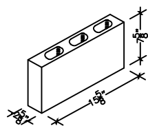
3" X 8" X 16" HOLLOW (ALSO IN 18")
