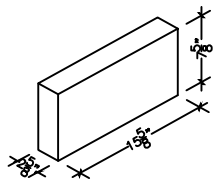
3" X 8" X 16" SOLID
