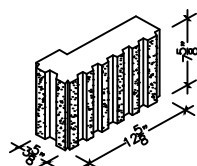
4" X 8" X 13" SOLID CORNER SPLIT RIB
