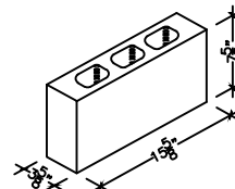
4" X 8" X 16" HOLLOW (ALSO IN 18")
