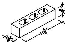
HALF HIGH 4" X 8" X 16" HOLLOW (ALSO IN 18")
