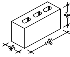
6" X 8" X 16" 75% SOLID (ALSO IN 18")
