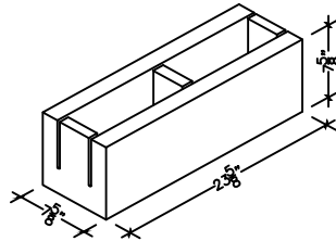
8" X 8" X 24" OPEN BOTTOM BOND BEAM (ALSO IN 18")
