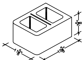
12" X 8" X 16" HOLLOW DOUBLE BULLNOSE (ALSO IN 18")
