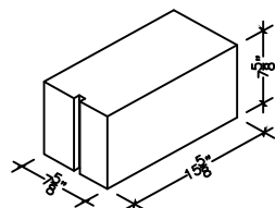
8" X 8" X 16" SOLID CORNER SASH
