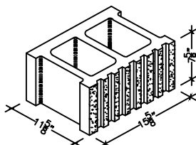
12" X 8" X 16" HOLLOW STRETCHER SPLIT RIB
