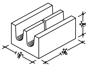
12" X 8" X 16" SOLID BOTTOM BOND BEAM (ALSO IN 18")
