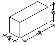
6" X 8" X 16" SOLID
