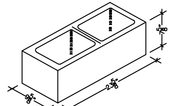
10" X 8" X 24" HOLLOW STRETCHER
