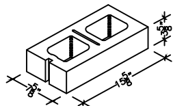
HALF HIGH 8" X 4" X 16" HOLLOW CORNER SASH (ALSO IN 18")
