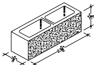
8" X 8" X 24" HOLLOW SPLIT FACE
