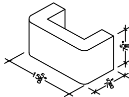
8" X 8" X 16" COLUMN COVER
