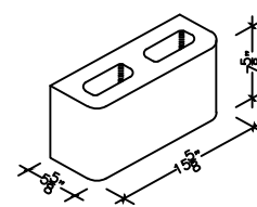
6" X 8" X 16" HOLLOW DOUBLE BULLNOSE (ALSO IN 18")
