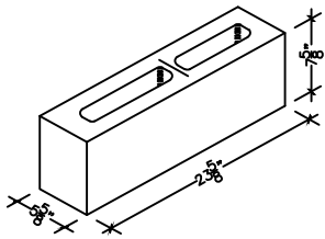
6" X 8" X 24" HOLLOW STRETCHER
