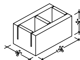
10" X 8" X 16" OPEN BOTTOM BOND BEAM (ALSO IN 18")
