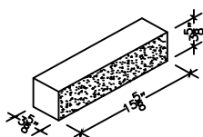
HALF HIGH 4" X 4" X 16" SPLIT FACE
