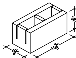
8" X 8" X 16" OPEN BOTTOM BOND BEAM (ALSO IN 18")
