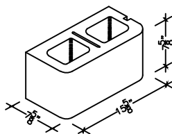
8" X 8" X 16" HOLLOW DOUBLE BULLNOSE (ALSO IN 18")
