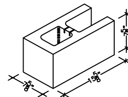
8" X 8" X 16" A SHAPED BLOCK (ALSO IN 18")
