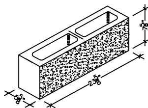
6" X 8" X 24" HOLLOW SPLIT FACE
