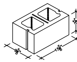
10" X 8" X 16" HOLLOW DOUBLE CORNER SASH (ALSO IN 18")
