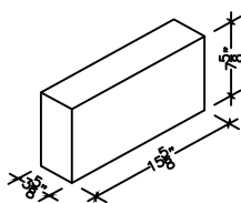
4" X 8" X 16" SOLID (ALSO IN 18")
