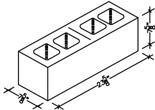
8" X 8" X 24" HOLLOW DOUBLE END ( 4 HOLE )
