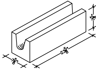
8" X 8" X 24" SOLID BOTTOM BOND BEAM (ALSO IN 18")
