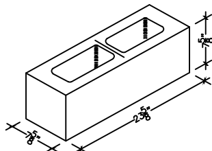
8" X 8" X 24" HOLLOW STRETCHER
