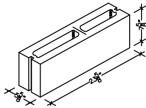
6" X 8" X 24" HOLLOW DOUBLE CORNER SASH
