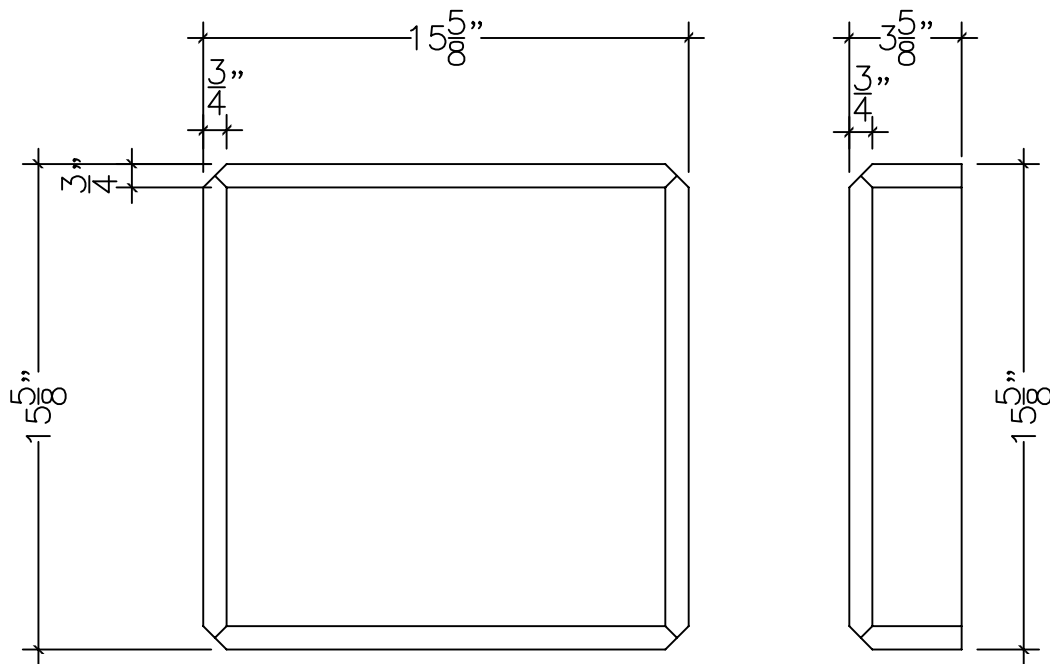
2 PC QUOIN CORNER ASSEMBLY
