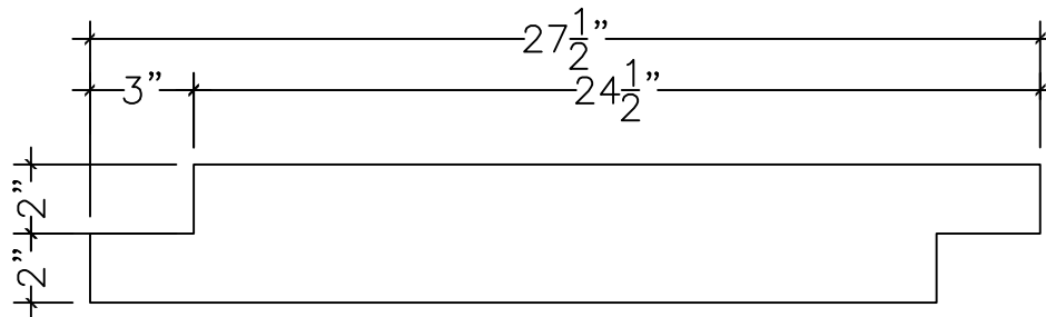
2 x 5 LAPLOCK COVER
