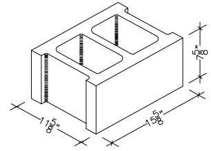
12" X 8" X 16" HOLLOW STRETCHER (ALSO IN 18")
