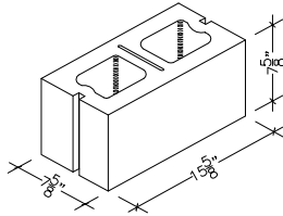
8" X 8" X 16" HOLLOW DOUBLE CORNER SASH (ALSO IN 18")
