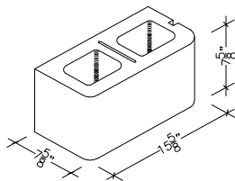
8" X 8" X 16" HOLLOW DOUBLE BULLNOSE (ALSO IN 18")
