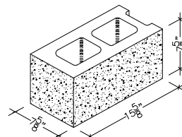
8" X 8" X 16" HOLLOW CORNER SPLIT FACE
