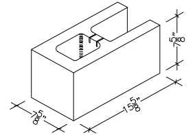
8" X 8" X 16" A SHAPED BLOCK (ALSO IN 18")
