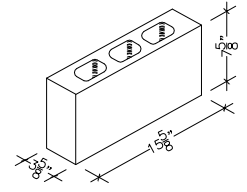
4" X 8" X 16" HOLLOW (ALSO IN 18")
