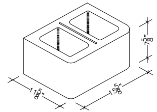
12" X 8" X 16" HOLLOW DOUBLE BULLNOSE (ALSO IN 18")
