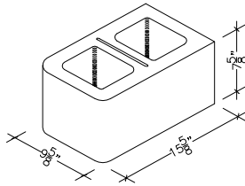
10" X 8" X 16" HOLLOW SINGLE BULLNOSE PIER (ALSO IN 18")
