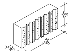
4" X 8" X 16" SOLID STRETCHER SPLIT RIB
