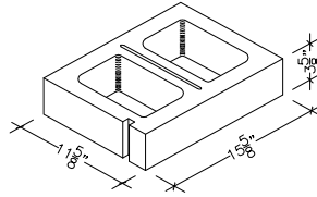
HALF HIGH 12" X 4" X 16" HOLLOW CORNER SASH (ALSO IN 18")
