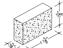
4" X 8" X 12" CORNER SPLIT FACE
