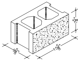
10" X 8" X 16" HOLLOW STRETCHER SPLIT FACE (ALSO IN 18")
