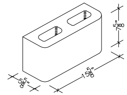
6" X 8" X 16" HOLLOW DOUBLE BULLNOSE (ALSO IN 18")
